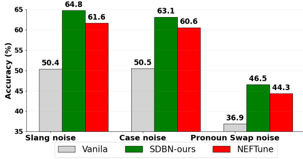
Figure 7: Adversarial training for constant-intensity noise. Performance comparison of BitFit PEFT implementations under constant-intensity noise conditions with DeBERTa-v3 on 1,000 samples from the Banking77 dataset. These results demonstrate the superior robustness of gradient-based adversarial training in low-resource settings.
