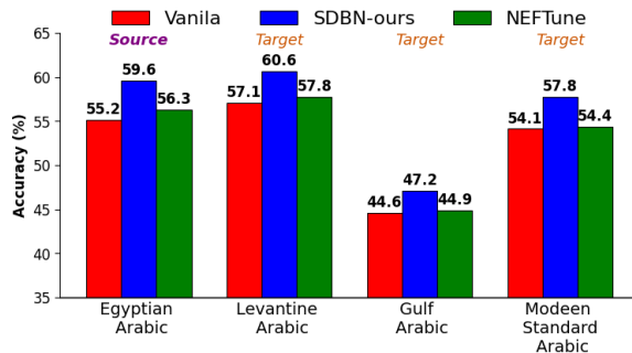
Figure 14: Domain Shifts. Comparison of LoRA PEFT methods on Arabic dialect sentiment classification using multilingual BERT-base trained on 270 samples of Egyptian Arabic without exposure to the other dialects during training. SDBN consistently outperforms alternatives across all dialects, with notable advantages on both the source and target domains.
