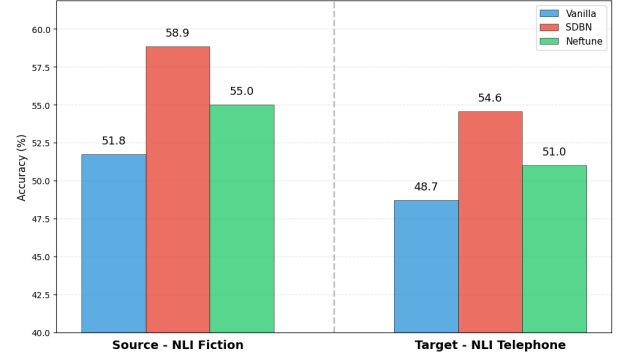
Figure 15: NLI Classification Performance: Source vs Target Domains. Performance comparison of LoRA PEFT methods on NLI classification tasks using DeBERTa-v3-large trained on only 77 samples from the source domain (NLI Fiction) without exposure to the target domain during training. Results show mean classification accuracy across 20 random seeds. SDBN consistently outperforms both vanilla LoRA and NEFTune across both domains, demonstrating superior robustness and generalization in this text classification scenario. While NEFTune shows improvement over vanilla LoRA through random noise injection, SDBN’s gradient-based adversarial perturbations provide more robustness, particularly valuable in this extreme low-resource classification setting.
