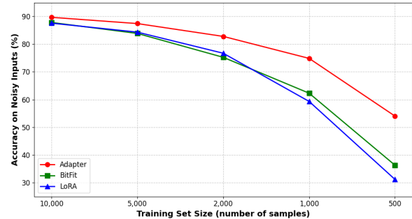
Figure 1: Performance degradation of PEFT methods on limited training data. Accuracy of three common PEFT methods: Adapter, BitFit, and LoRA—on a test set with word-swapping noise as the size of the clean Banking77 training data corpus is reduced (x-axis, number of examples). All methods exhibit a marked drop in noisy-test accuracy as the available training data dwindles , in some cases losing more than 50% below 1,000 training samples. The trend underscores the current vulnerability of PEFT models to realistic textual perturbations in low-resource settings.
